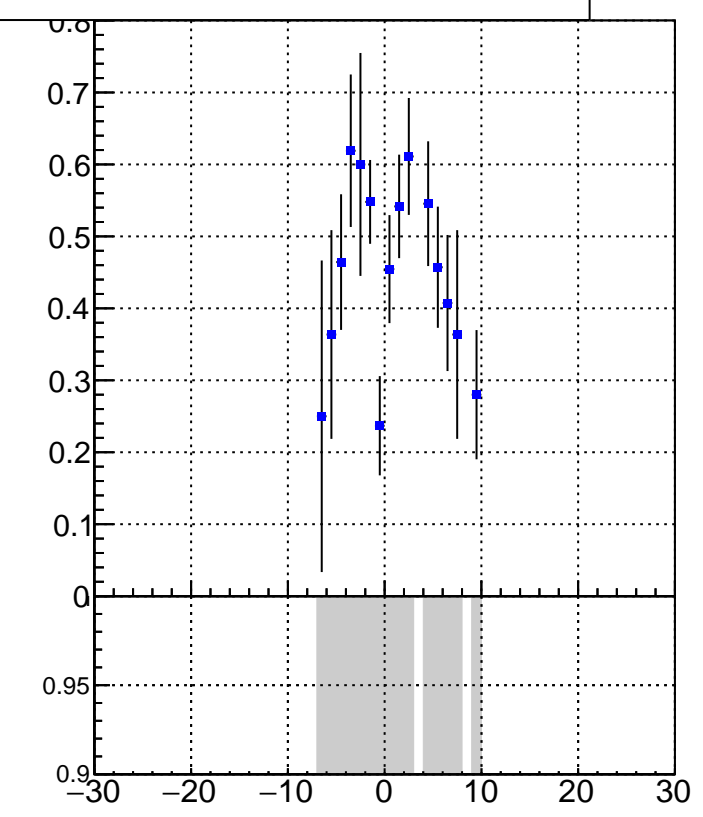
—■ DQM_V0001_R000000001_Global_CMSSW_X_Y_Z_RECO
