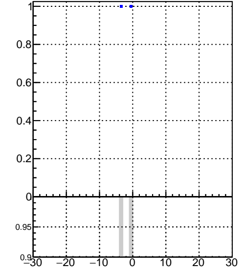
Efficiency vs vertpos Legend: DQM_V0001_R000000001_Global_CMSSW_X.Y.Z_RECO
