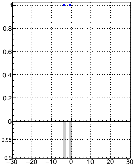
Fake rate vs dxy DQM_V0001_R000000001_Global_CMSSW_X_Y_Z_RECO
