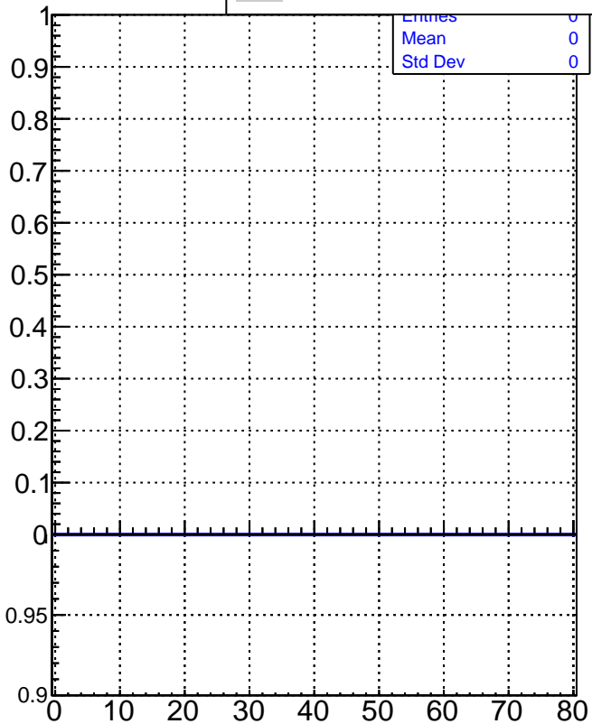
DQM_V0001_R000000001_Global_CMSSW_X_Y_Z_RECO
