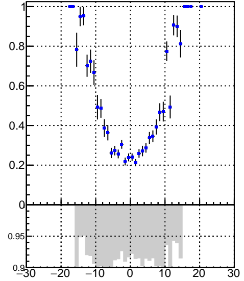
Efficiency vs sim PV z | fake+duplicates vs Sim. PV z Legend: DQM_V0001_R000000001_Global_CMSSW_X.Y.Z_RECO
