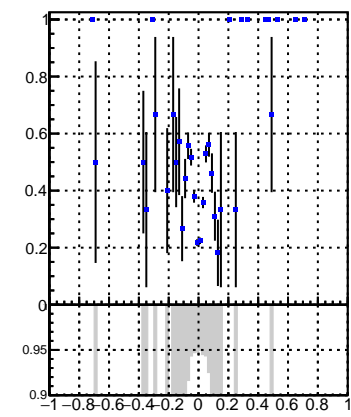
Fake rate vs d DQM_V0001_R000000001_Global_CMSSW_X_Y_Z_RECO
