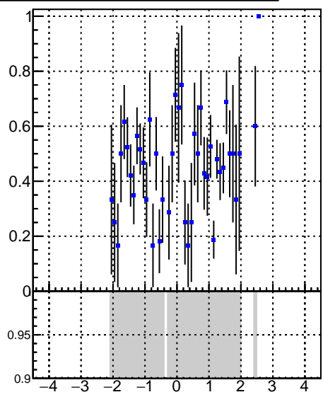
Legend: DQM_V0001_R000000001_Global_CMSSW_X_Y_Z_RECO
