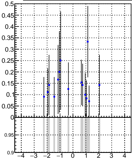
Legend: DQM_V0001_R000000001_Global_CMSSW_X_Y_Z_RECO
