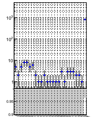
recoToSim
