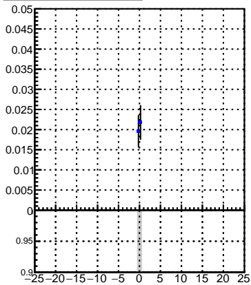
Efficiency ● DQM_V0001_R000000001_Global_CMSSW_X_Y_Z_RECO
