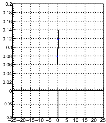
Efficiency ● DQM_V0001_R000000001_Global_CMSSW_X_Y_Z_RECO
