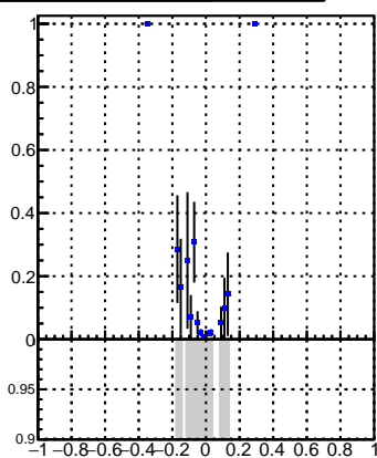
Efficiency ● DQM_V0001_R000000001_Global_CMSSW_X_Y_Z_RECO
