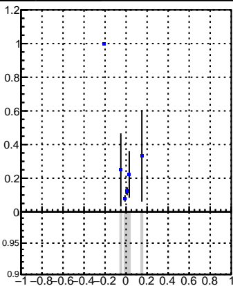
Efficiency ● DQM_V0001_R000000001_Global_CMSSW_X_Y_Z_RECO
