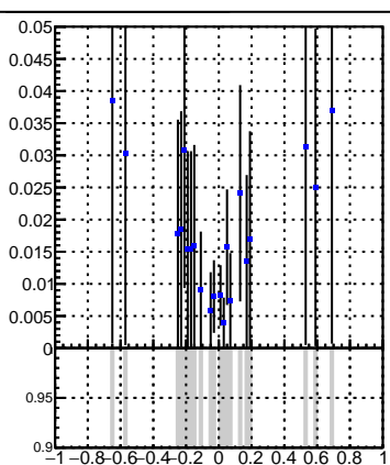
DQM_V0001_R000000001_Global_CMSSW_X_Y_Z_RECO
