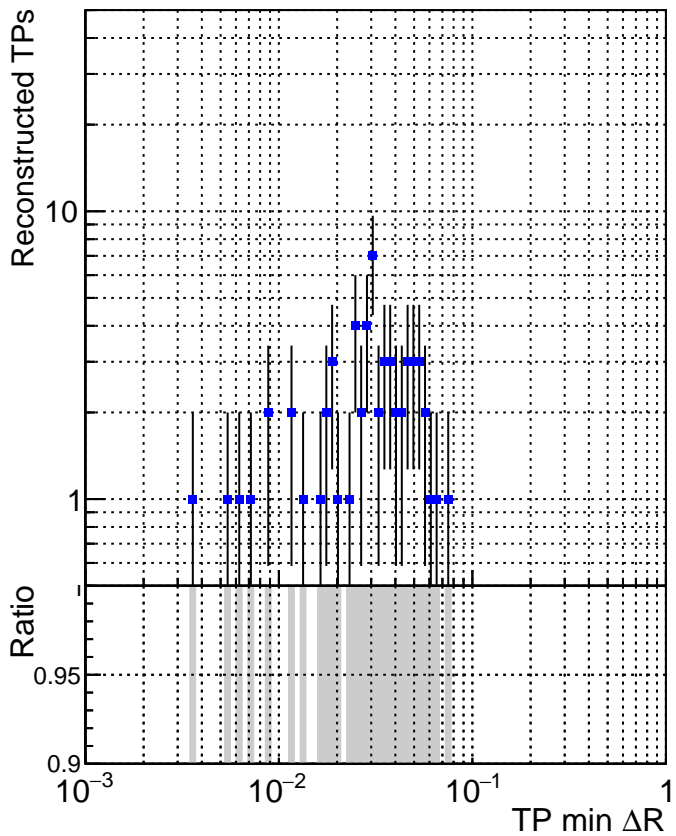
■ DQM_V0001_R000000001_Global_CMSSW_X_Y_Z_RECO
