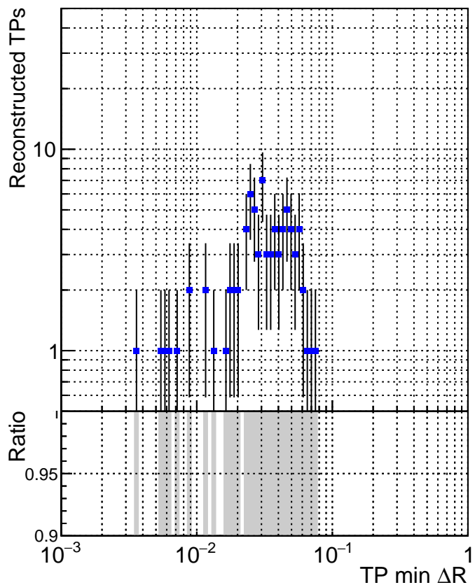
Legend: DQM_V0001_R000000001_Global_CMSSW_X_Y_Z_RECO
