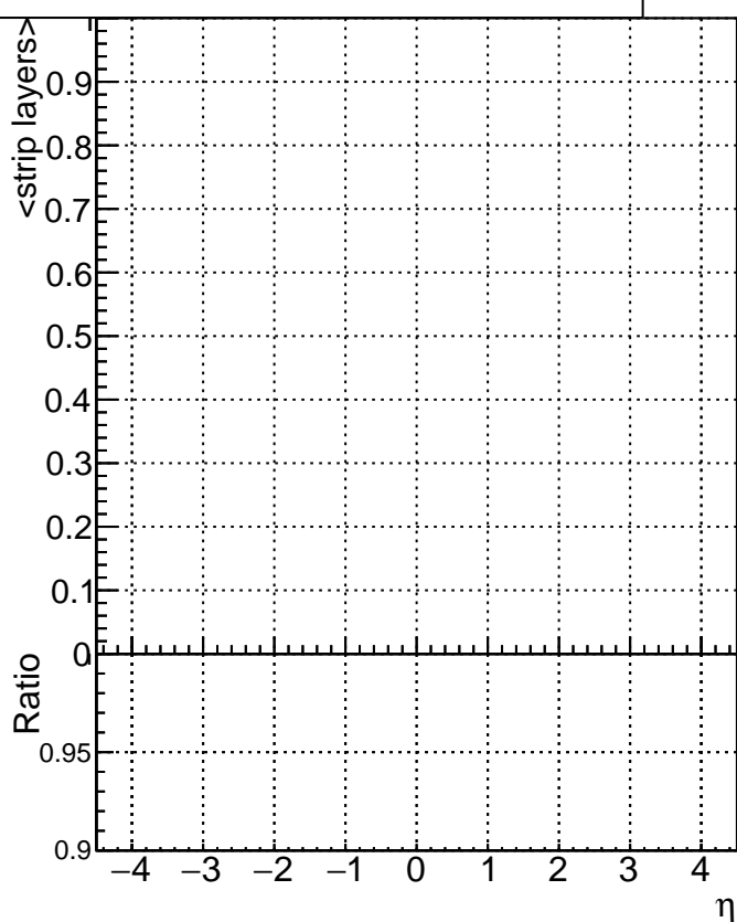
DQM_V0001_R000000001_Global_CMSSW_X_Y_Z_RECO
