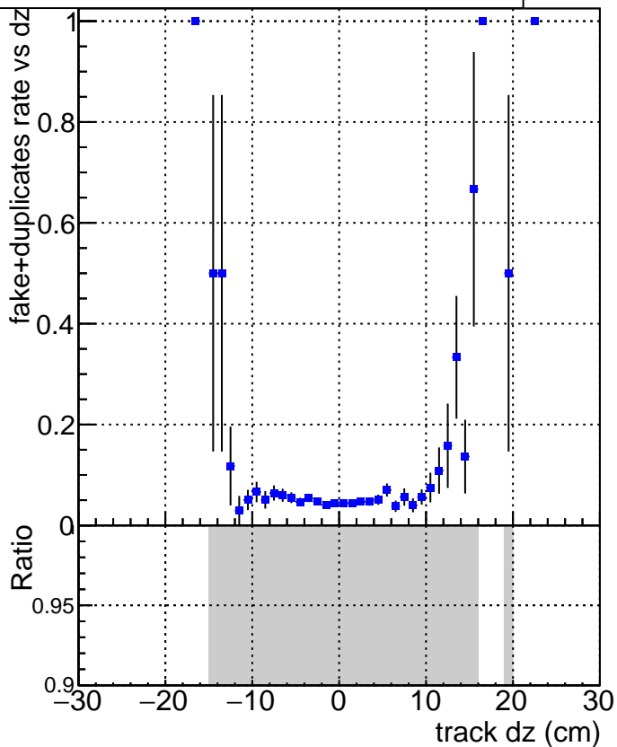
DQM_V0001_R000000001_Global_CMSSW_X_Y_Z_RECO
