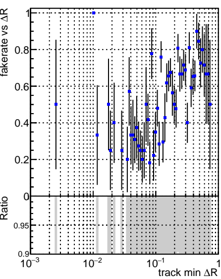
Fake rate vs \Delta R(\text{track, jet}) DQM_V0001_R00000001_Global_CMSSW_X_Y_Z_RECO
