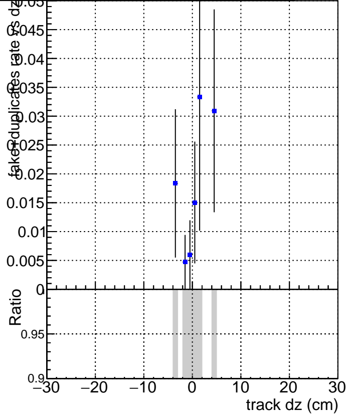
DQM_V0001_R000000001_Global_CMSSW_X_Y_Z_RECO
