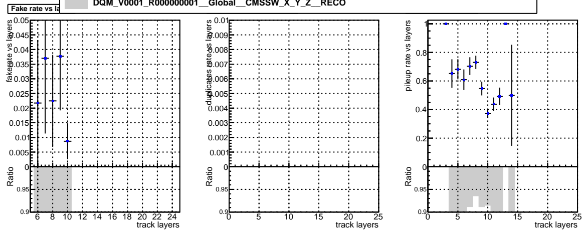
DQM_V0001_R000000001_Global_CMSSW_X_Y_Z_RECO
