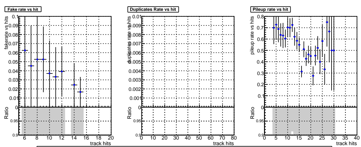
DQM_V0001_R000000001_Global_CMSSW_X_Y_Z_RECO
