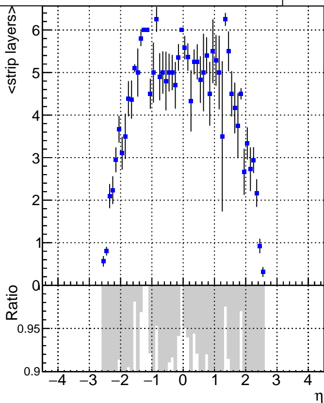
DQM_V0001_R000000001_Global_CMSSW_X_Y_Z_RECO
