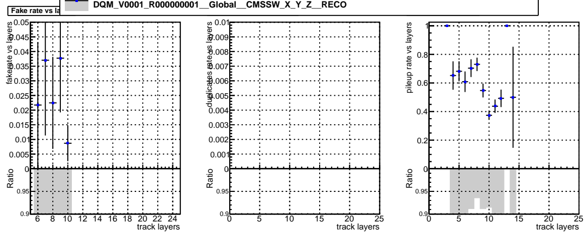
DQM_V0001_R000000001_Global_CMSSW_X_Y_Z_RECO
