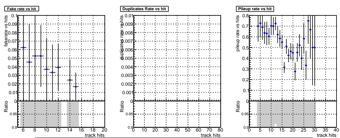
DQM_V0001_R000000001_Global_CMSSW_X_Y_Z_RECO
