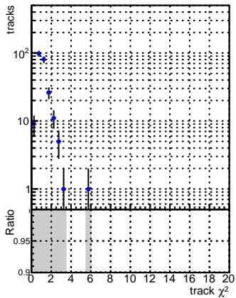
N of reco track vs. DQM_V0001_R000000001_Global_CMSSW_X_Y_Z_RECO
