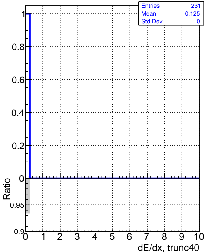
DQM_V0001_R000000001_Global_CMSSW_X_Y_Z_RECO
