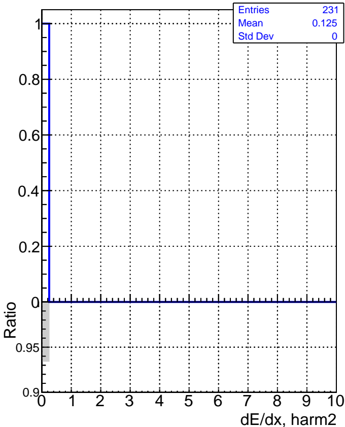
DQM_V0001_R000000001_Global_CMSSW_X_Y_Z_RECO
