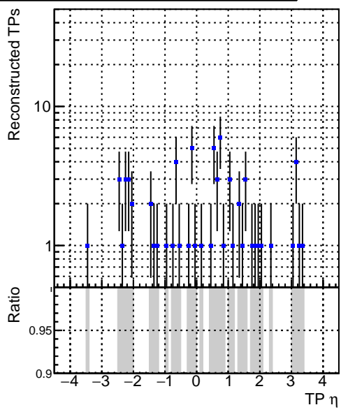
■ N of simulated tracks ■ DQM_V0001_R000000001_Global_CMSSW_X_Y_Z_RECO
