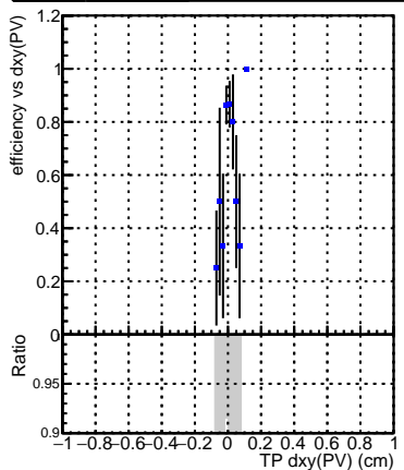
Efficiency vs Dxy(PV) DQM_V0001_R000000001_Global_CMSSW_X_Y_Z_RECO
