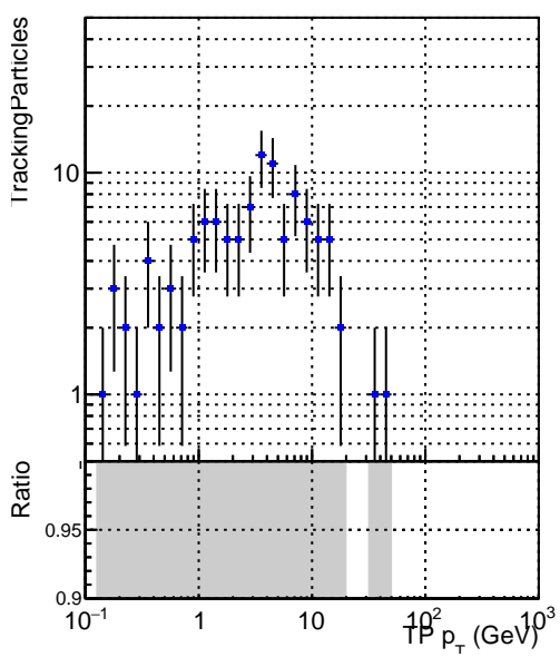
■ N of sim ■ DQM_V0001_R000000001_Global_CMSSW_X_Y_Z_RECO
