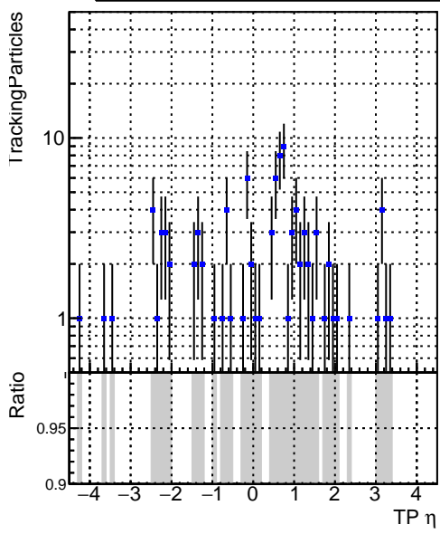
■ N of sim ■ DQM_V0001_R000000001_Global_CMSSW_X_Y_Z_RECO
