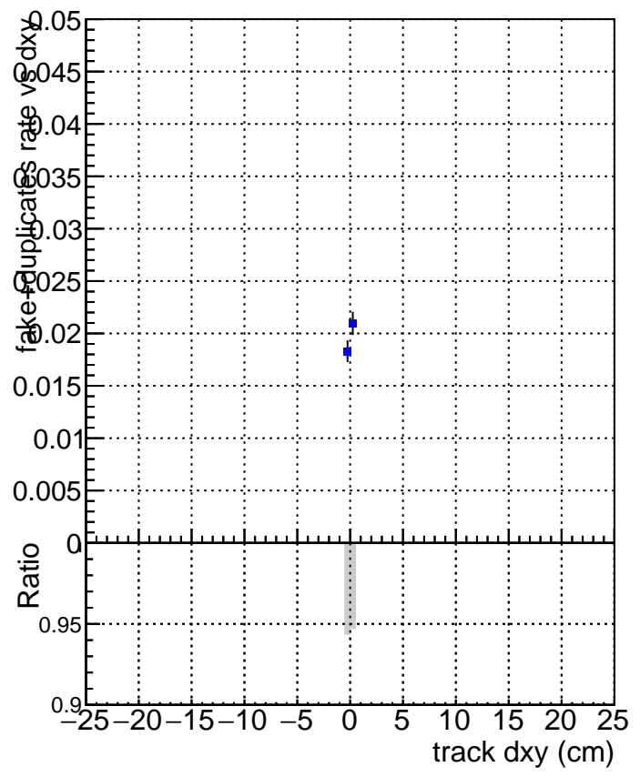
—■ DQM_V0001_R000000001_Global_CMSSW_X_Y_Z_RECO
