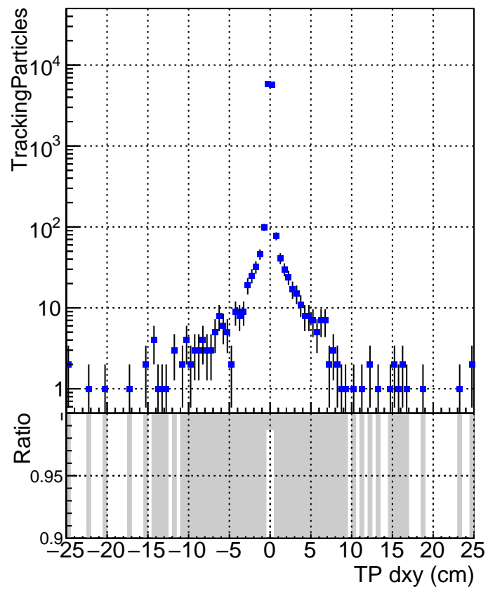
N of simulated track ■ DQM_V0001_R000000001_Global_CMSSW_X_Y_Z_RECO
