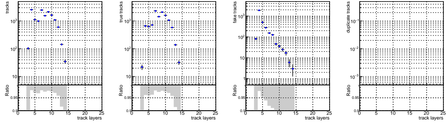
DQM_V0001_R000000001_Global_CMSSW_X_Y_Z_RECO
