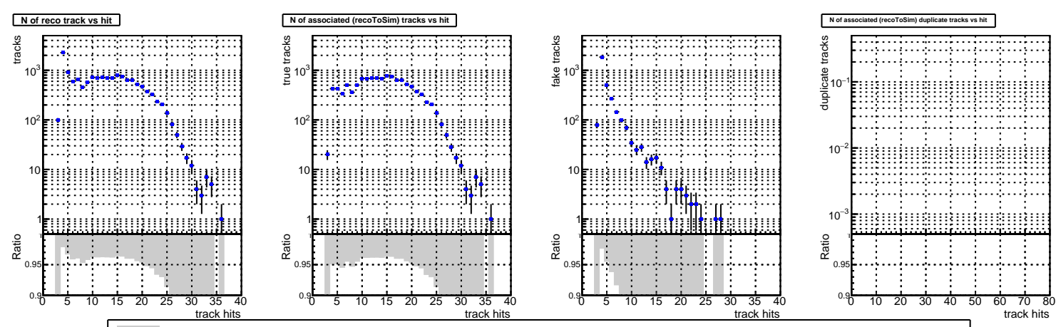
DQM_V0001_R000000001_Global_CMSW_X_Y_Z_RECO
