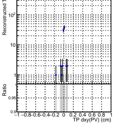
N of associated tracks (simToReco) vs dxy(PV)
