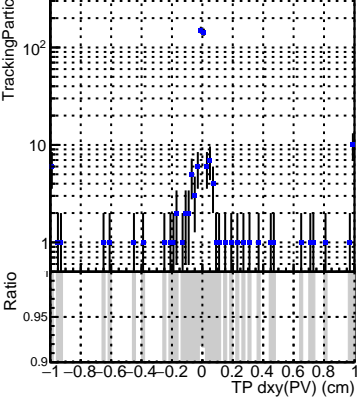
N of simulated tracks vs dxy(PV)
