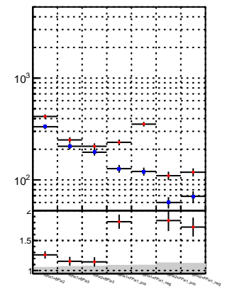
N of associated (recoToSim) looper tracks vs. \chi^2 oob trackingLST-rmlS-mask-8c1d76e
