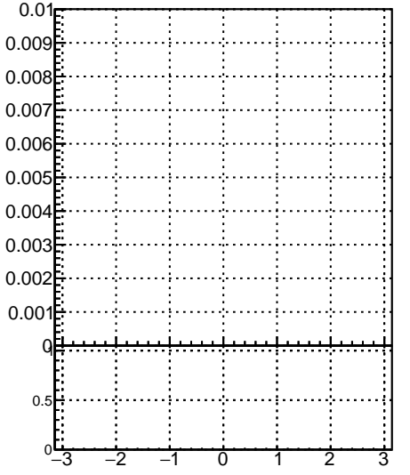
Fake rate vs \phi
