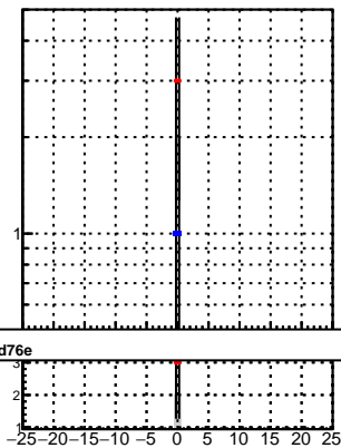
N of associated (recoToSim) tracks vs dxy
