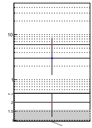
N of reco track vs. \chi^2 oob trackingLST-rmlS-mask-8c1d76e
