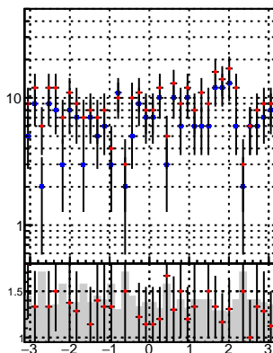
N of associated (recoToSim) tracks vs phi
