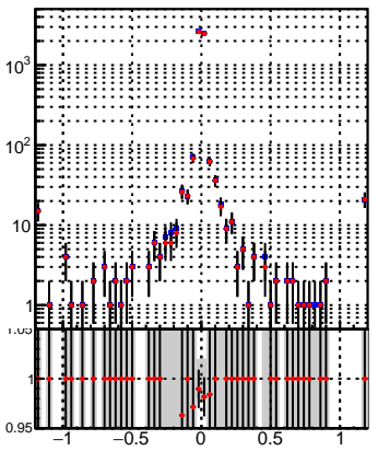
N of simulated tracks vs dz(PV) for trackingLST-rmIS-mask-8c1d76e
