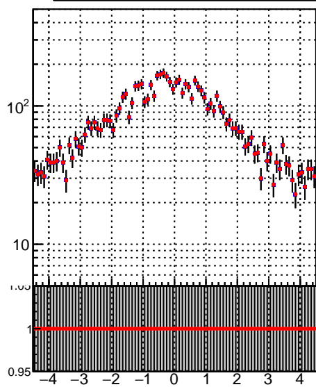
N of simulated tracks vs phi N of associated tracks (simToReco) vs phi Legend: oob (blue cross), trackingLST-rmlS-mask-8c1d76e (red cross)
