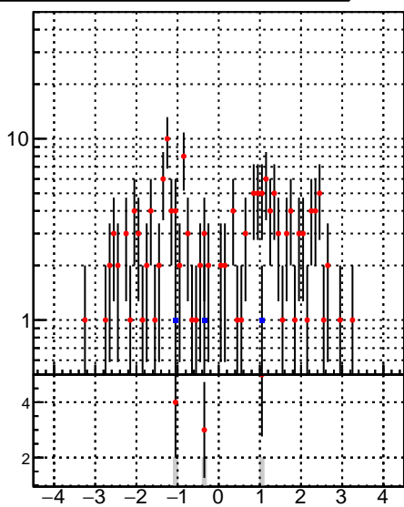
N of simulated tracks vs phi N of associated tracks (simToReco) vs phi Legend: oob (blue cross), trackingLST-rmlS-mask-8c1d76e (red cross)
