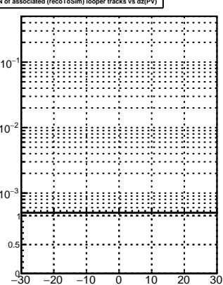
N of associated (recoToSim) looper tracks vs dz(PV)
