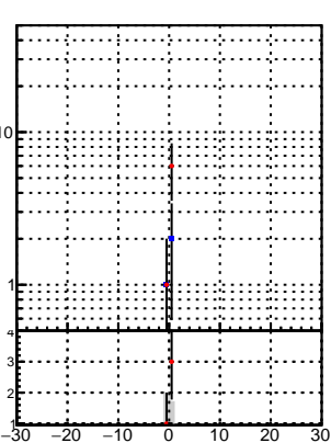
N of associated (recoToSim) tracks vs dz(PV)
