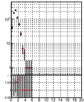
N of reco track vs. \chi^2 oob trackingLST-rmlS-mask-8c1d76e
