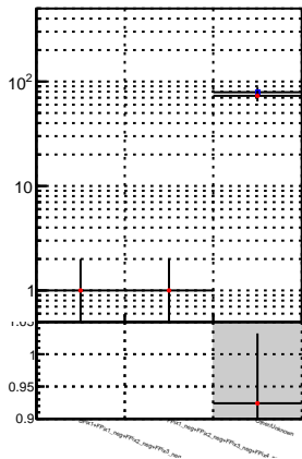
N of reco track vs. oob trackingLST-rmlS-mask-8c1d76e
