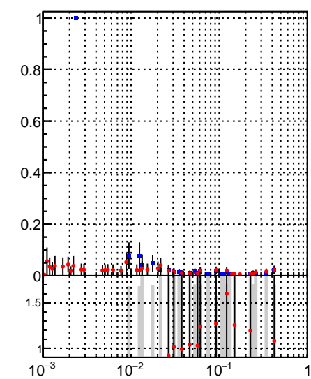
Fake rate vs oob Fake rate vs trackingLST-rmIS-mask-8c1d76e
