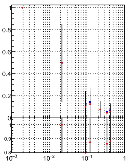
Fake rate vs oob Fake rate vs trackingLST-rmIS-mask-8c1d76e
