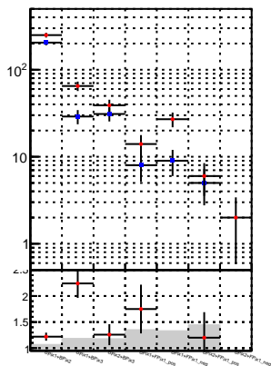
N of reco track vs. \chi^2 oob trackingLST-rmlS-mask-8c1d76e
