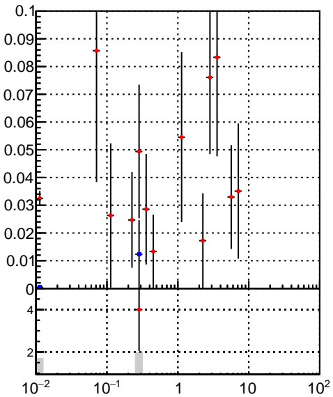
Efficiency vs sim PV z oob (blue square) trackingLST-rmlS-mask-8c1d76e (red circle)
