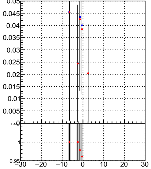
Efficiency vs sim PV z oob (blue square) trackingLST-rmlS-mask-8c1d76e (red circle)
