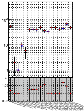
N of reco track vs. \chi^2 oob trackingLST-rmlS-mask-8c1d76e
