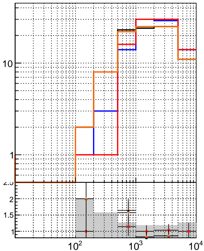
RecoAssoc2GenPVMatched_Pt2
