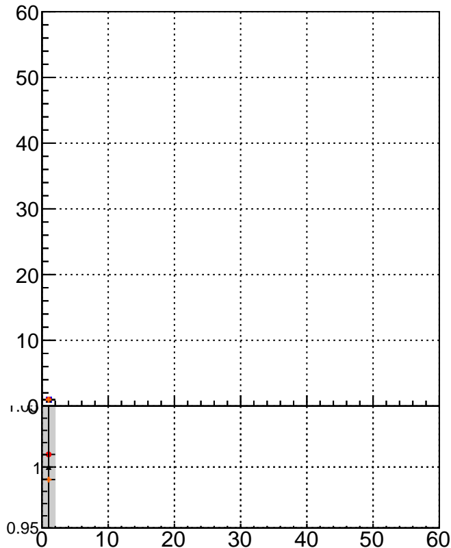
MatchedRecoVtx_vs_GenVtx
