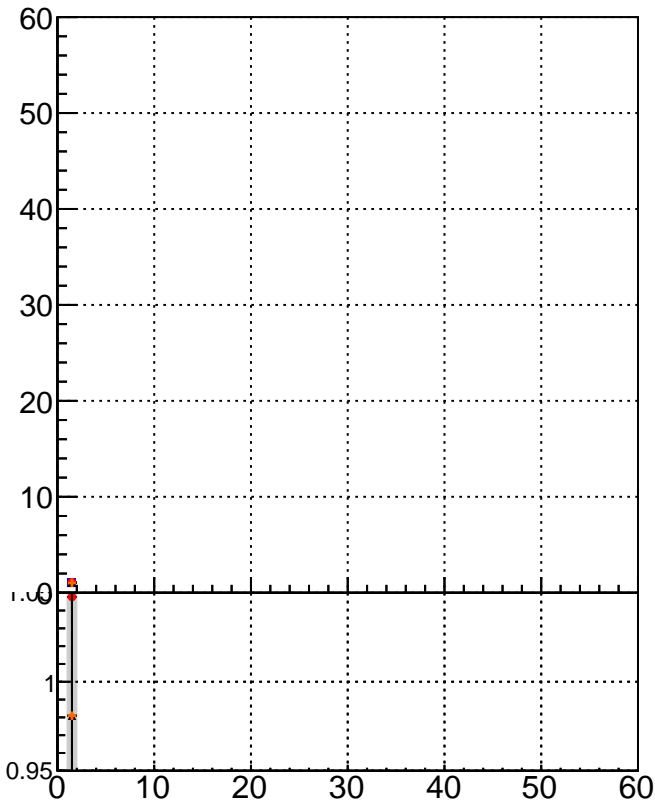
RecoVtx_vs_GenVtx
