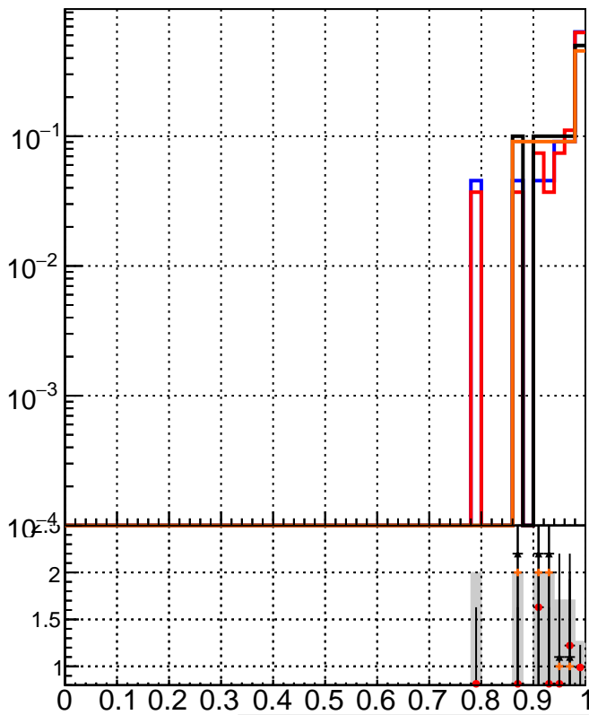
RecoPVAssoc2GenPVMatched_Purity
