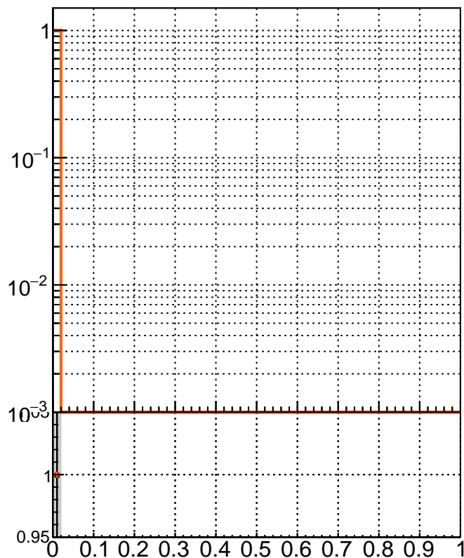
RecoPVAssoc2GenPVNotMatched_missing
