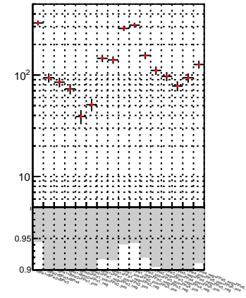
N of reco track vs. \chi^2 oob
