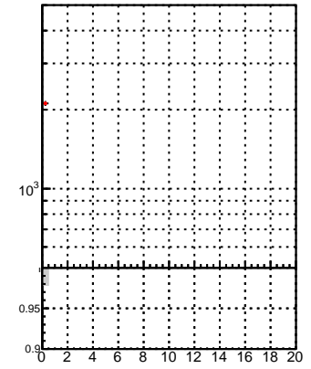
N of associated (recoToSim) tracks vs. \chi^2 oob
