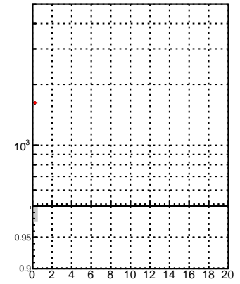
N of associated (recoToSim) looper tracks vs. \chi^2 oob
