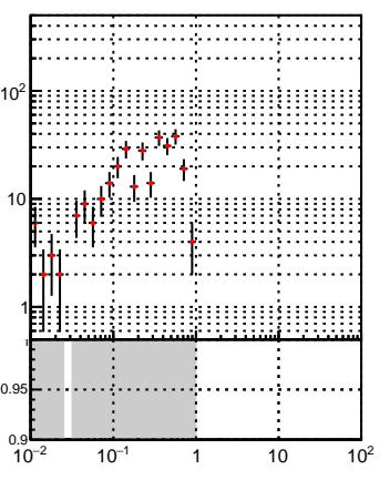
N of associated (recoToSim) loopers vs transverse ref point position
